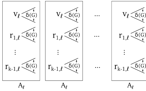
Figure 5.2: Sketch of the setting of Lemma 4 and Theorem 4. (v_1, \dots, v_\ell) is a path in a graph G , and each set A_i contains the vertex v_i and k - 1 other vertices r_{1,i}, \dots, r_{k-1,i} . Each of those vertices has an outdegree of at least \delta(G) .
