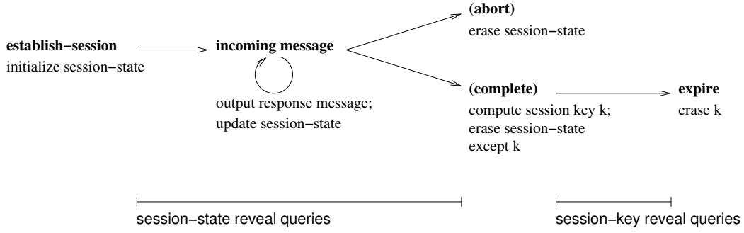
Figure 1: Lifetime of a session in CK. Although session-state reveal queries are allowed after the session is completed, the returned state will be empty [5, p. 11], and we omit these from the graph.
