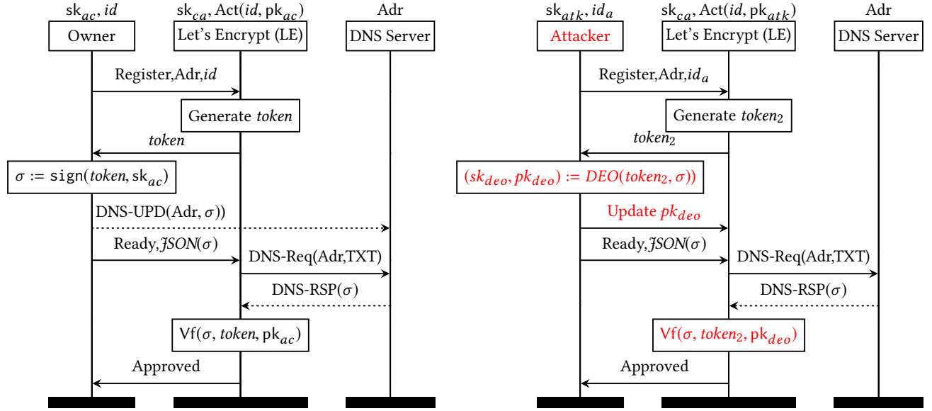
(a) Normal Operation of the Automatic Certificate Management Environment (ACME) Draft 00 Protocol
