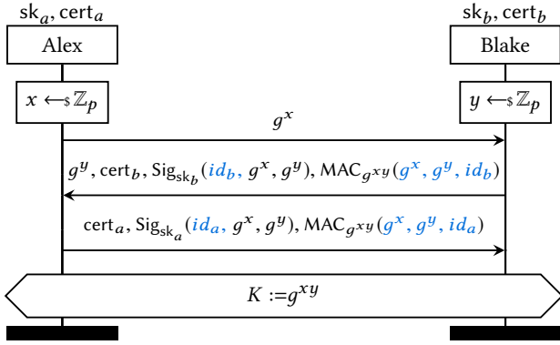
Figure 3: Sketch of STS-ISO [37], which includes the identities of the communicating parties.
