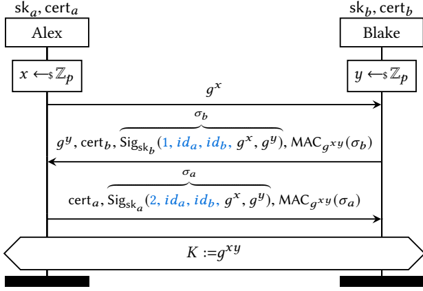
Figure 2: Sketch of STS-ID [37], which includes the identities of the communicating parties in the MAC.
