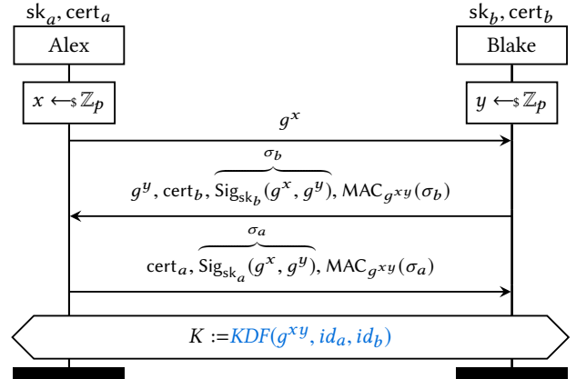
Figure 6: Sketch of STS-KDF [37], which patches STS-MAC by including the identities of the communicating parties in the KDF.
