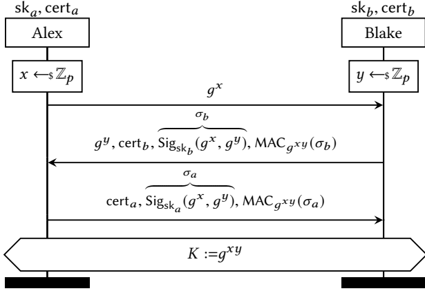
Figure 1: Sketch of the original STS-MAC protocol [50]
