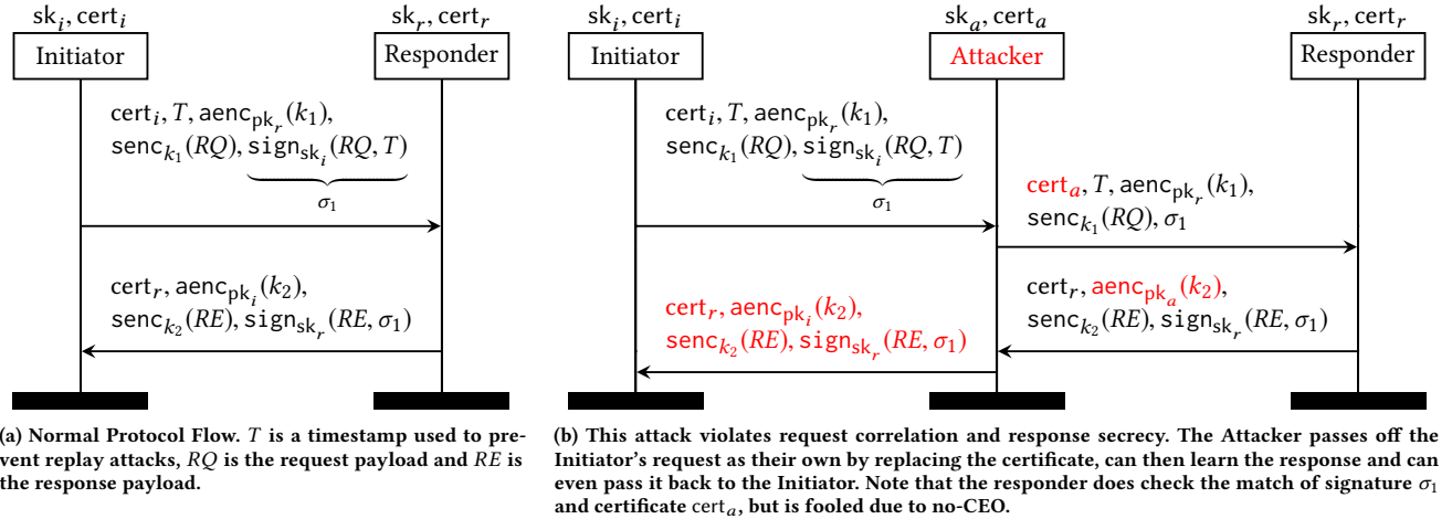
Figure 8: The WSS1.1-MA-X509-SE protocol from [19] and the attack we automatically discovered.
