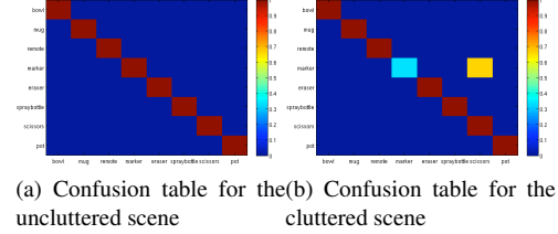
Figure 5: Categorization confusion tables for detected object
